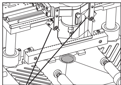
Double lubrication of the tool
